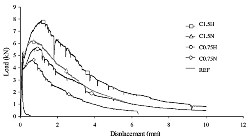
Figure (1): Ackay & Tasdemir curves of load-displacement for five mixes [14].
