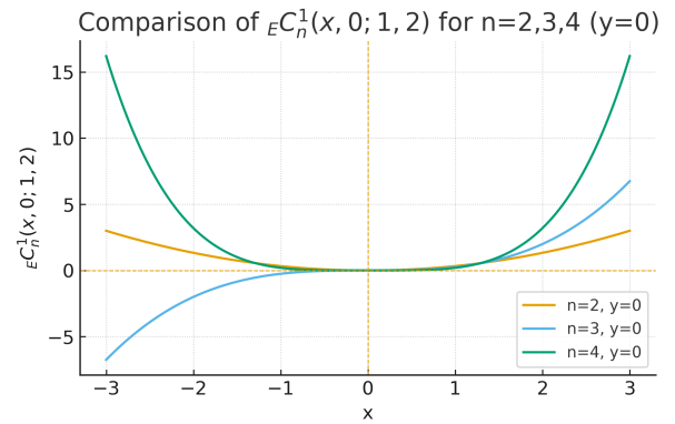
Figure 4: Comparison of {}_EC_n^1(x, 0; 1, 2) for n = 2, 3, 4 .
