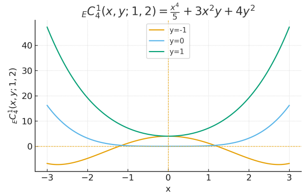
Figure 3: Graph of {}_EC_4^1(x, y; 1, 2) = \frac{x^4}{5} + 3x^2y + 4y^2 .
