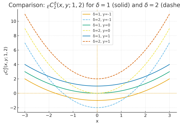
Figure 5: Plots of {}_EC_2^\delta(x, y; 1, 2) for \delta = 1 and 2 at y = -1, 0, 1 .
