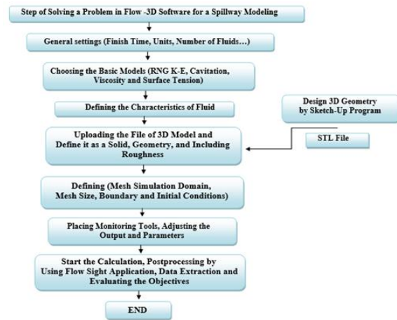
Figure (6): The Flow-3D program has a spillway modeling methodology.
