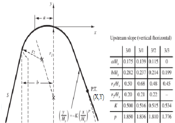
Figure (4): Spillway crest profile.
