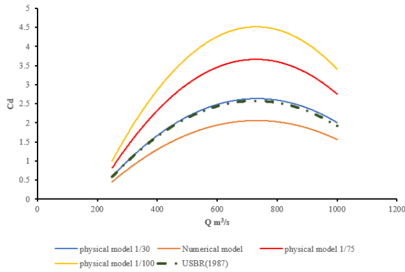
Figure (10): The discharge coefficients compare physical models, numerical model, and USBR (1987).
