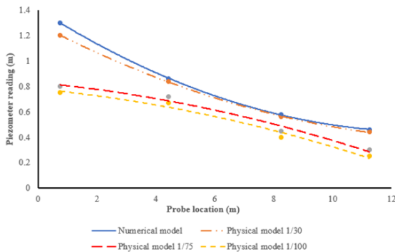
Figure (12): Piezometer reading the comparison between physical models and numerical model in discharge 500 m³/s.
