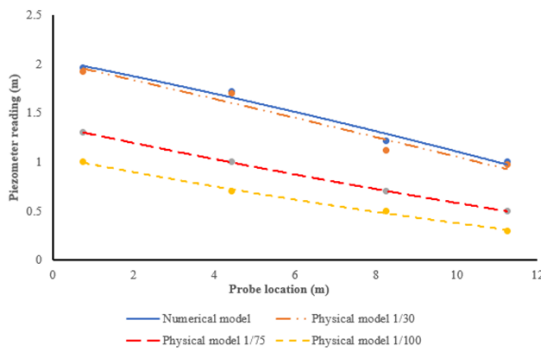
Figure (13): Piezometer reading the comparison between physical models and numerical model in discharge 1000 m³/s.
