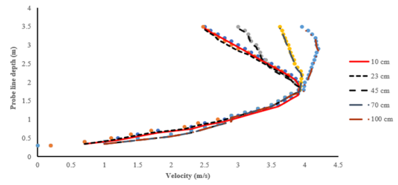
Figure (14): A second-order fit curve for the distribution of velocities at the spillway crest.
