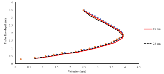
Figure (15): Flow-3D software's velocity sensitivity study for 23 and 10 cm mesh sizes.
