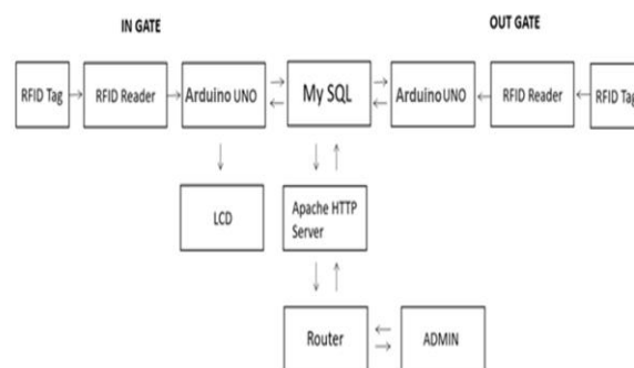
Figure (4): Block Diagram of RFID - based authentication module.
