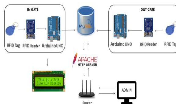
Figure (5): Functional Diagram of RFID based authentication model.
