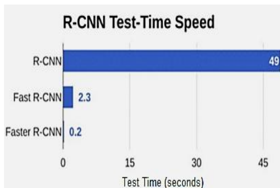
Figure (3): Comparison of object detection algorithms [7].
