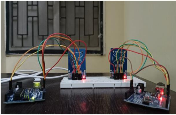
Figure (9): Experimental setup for gate module.
