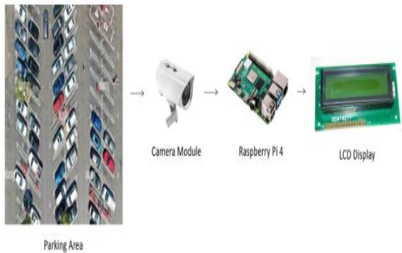
Figure (7): Functional Diagram of parking slot detection module.
