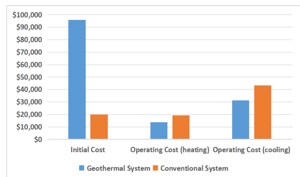
Figure (3): Initial and operating cost (heating and cooling) for the geothermal and conventional systems.
