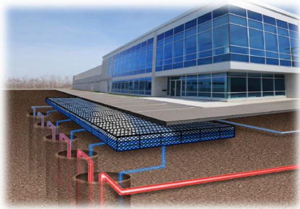
Figure (2): vertical loop system.
