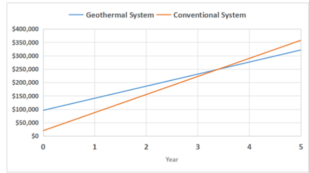
Figure (6): The break-even for the geothermal system.
