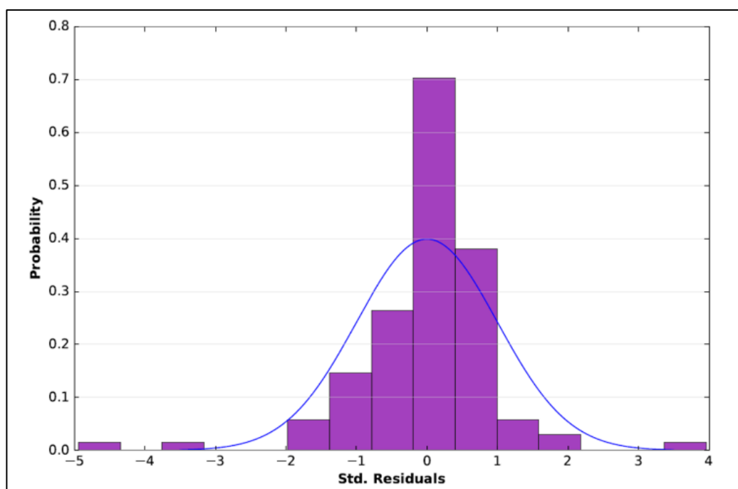
Figure (12): Histogram of standardized residuals.
