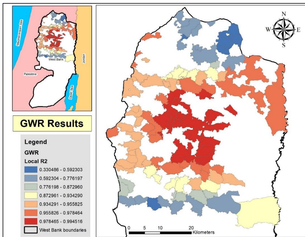
Figure (10): Geographic Weighted Regression results – (Local R^2 ).
