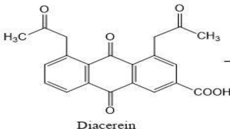
Figure (2): Chemical Structure of diacerein.
