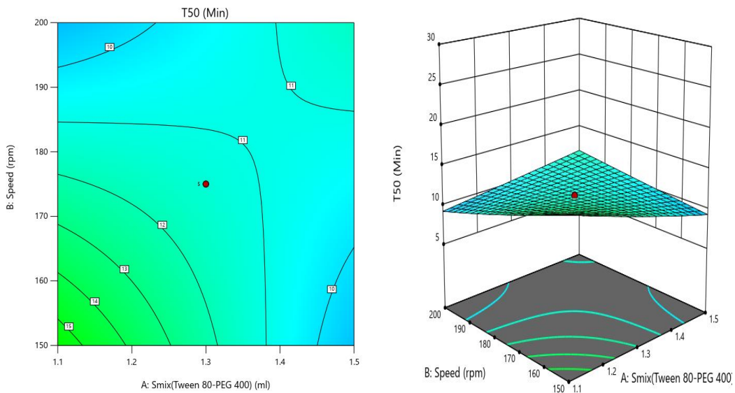
Figure (9): A. Counter plots of T50 B. 3D Surface Plots of T50
