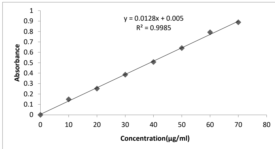
Figure (3): Calibration curve for the Estimation of Mirtazapine by using 0.1N Hydrochloric acid Buffer.
