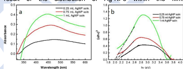
Figure (2): (a) UV-vis absorption spectra of prepared PVA / Ag nanocomposite Tauc plot of PVA / Ag nanocomposite at medium-high power.
