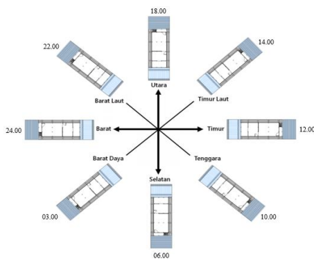
Figure (5): (a) Orientation of the Floating Houses, and (b) Shape of the Floating Houses Source: compiled by the authors
