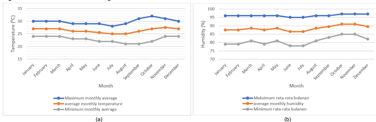
Figure (2): Climate Conditions at Lake Tempe (a) Air Temperature and (b) Relative Humidity
