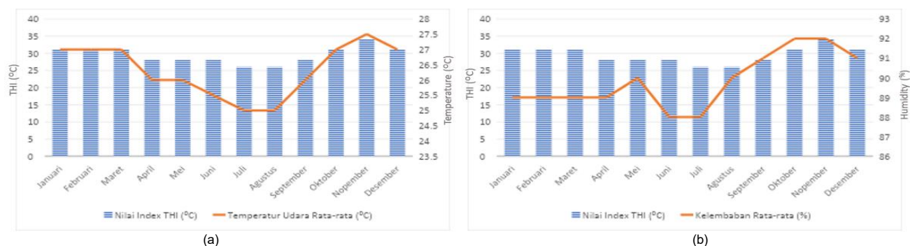
Figure (3): Relationship between (a) Average Air Temperature and THI Values, and (b) Average Relative Humidity and THI Values Source: compiled by the authors.
