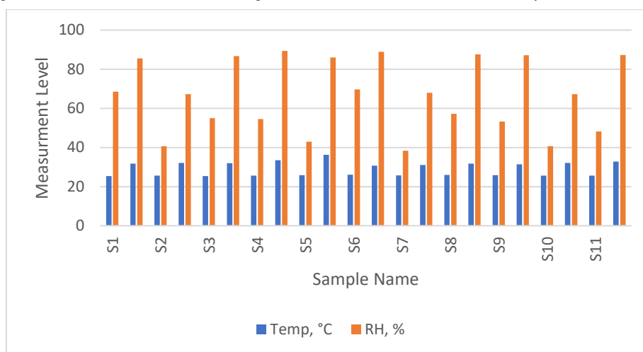
Figure (4): Minimum and maximum Temperature and Humidity values for each research sample.
