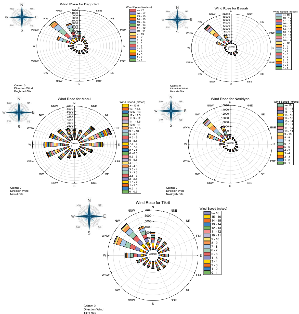
Figure (6): Wind rose at the selected sites.
