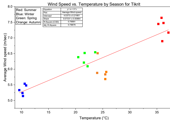
Figure (7): Scatter plot of wind speed vs. temperature for selected sites.
