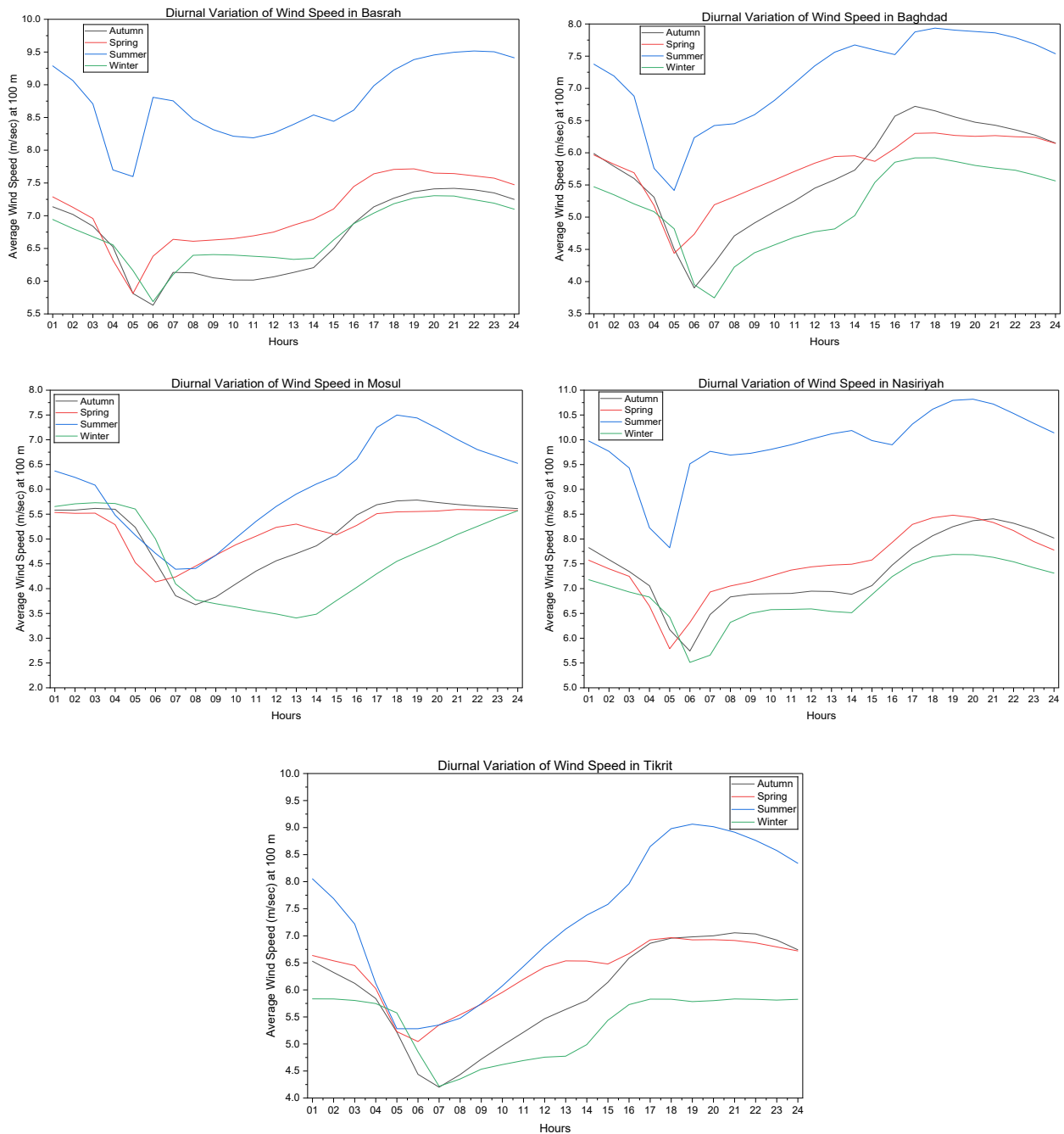
Figure (4): Average diurnal wind speed in summer for selected sites.
