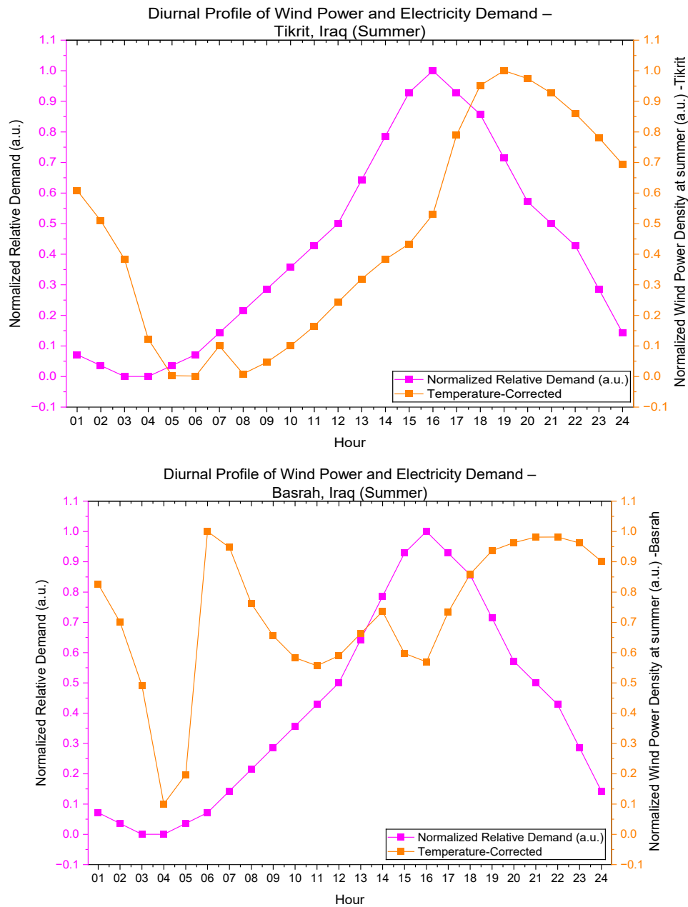
Figure (5): Hourly Normalized Wind Power Density vs. Electrical Demand Multiplier (Summer Months).
