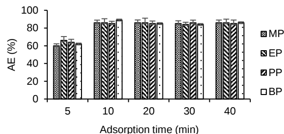
Figure 1b. Influence of adsorption time on adsorption efficiency. Standard deviations are plotted as error bars.
