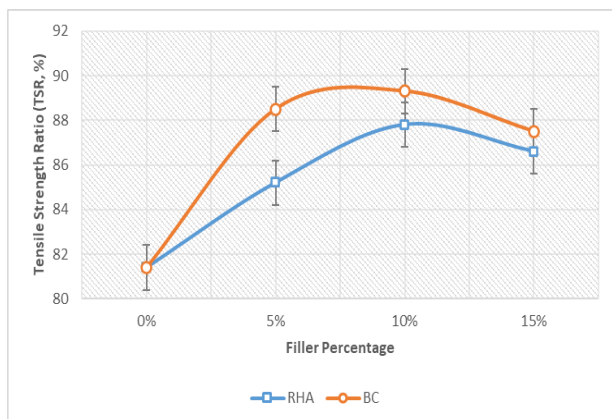
Figure (7): Tensile Strength Ratio Results
