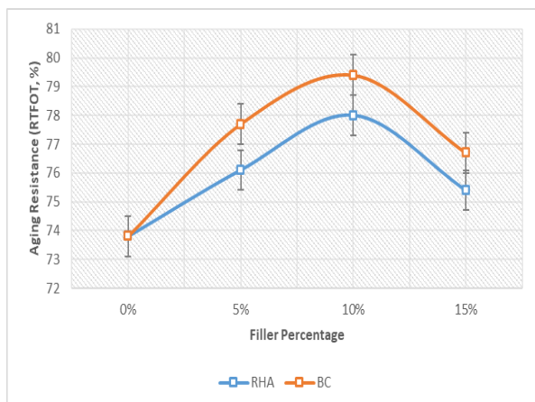
Figure (8): Aging Resistance (RTFOT) Results.
