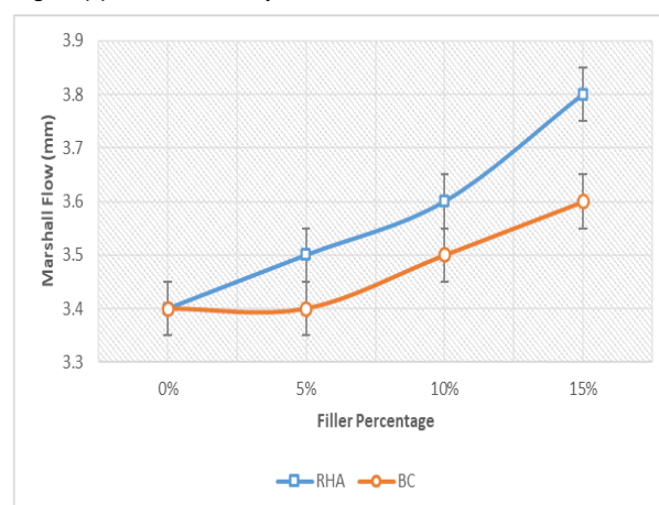
Figure (2): Marshall Flow Results.
