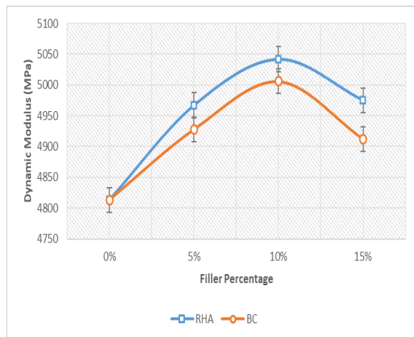
Figure (3): Dynamic Modulus Results.
