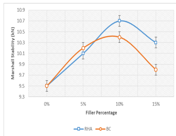
Figure (1): Marshall Stability Results.
