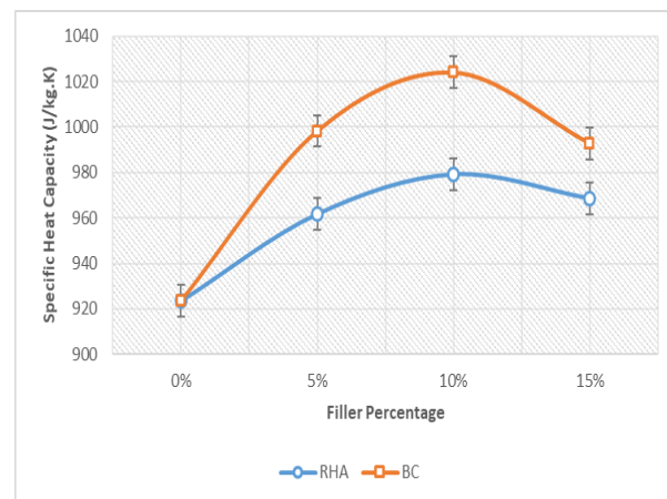
Figure (6): Specific Heat Capacity Results
