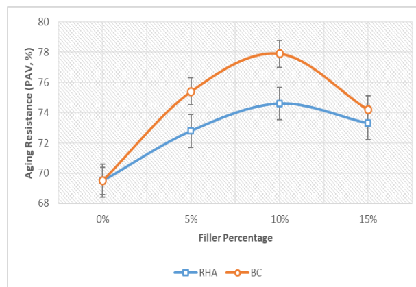
Figure (9): Aging Resistance (PAV) Results.
