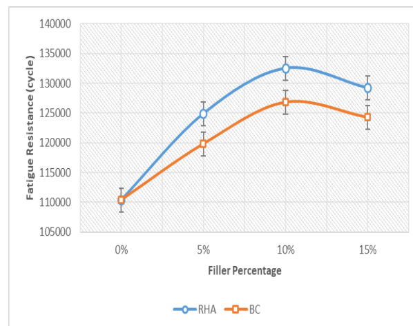
Figure (4): Fatigue Resistance Results
