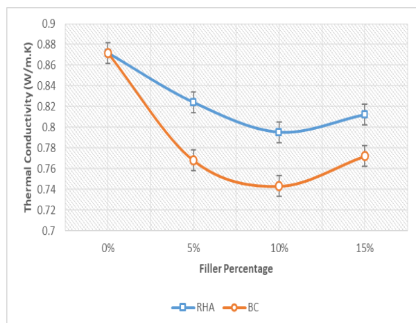
Figure (5): Thermal Conductivity Results
