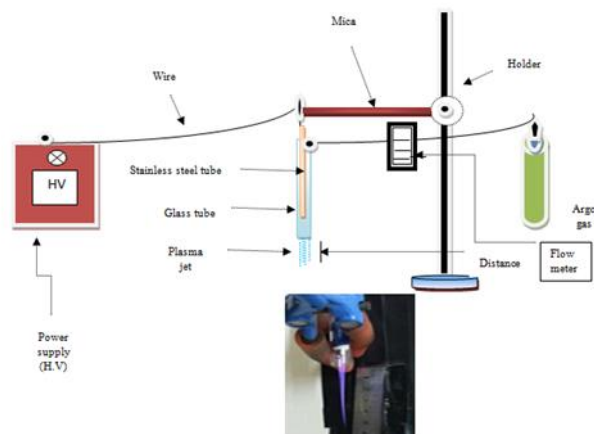
Figure 1 : Torch plasma
