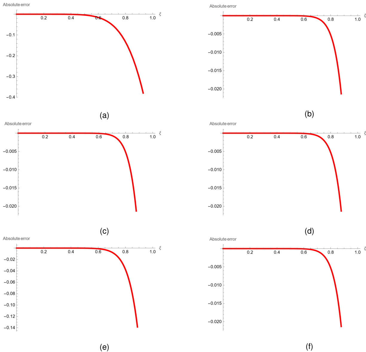
Figure (2): The obtained results exhibit strong and satisfactory convergence towards the exact solution affirming the high quality of performance and robustness of the proposed algorithm by the MADM ( L_1 - L_6 ).
