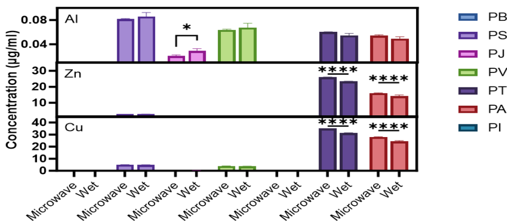
Figure (2): Concentrations ( \mu\text{g/mL} ) of Al, Zn, and Cu in seven natural oil products from different origins. All samples were analyzed by ICP-OES spectrometer following their digestion with both the closed-microwave and the open-wet methods. Data points represent concentration mean \pm SD (n = 3). Significant differences between the closed-microwave and open-wet digestion methods for the same detected element are expressed as * P < 0.05 and **** P < 0.0001 .
