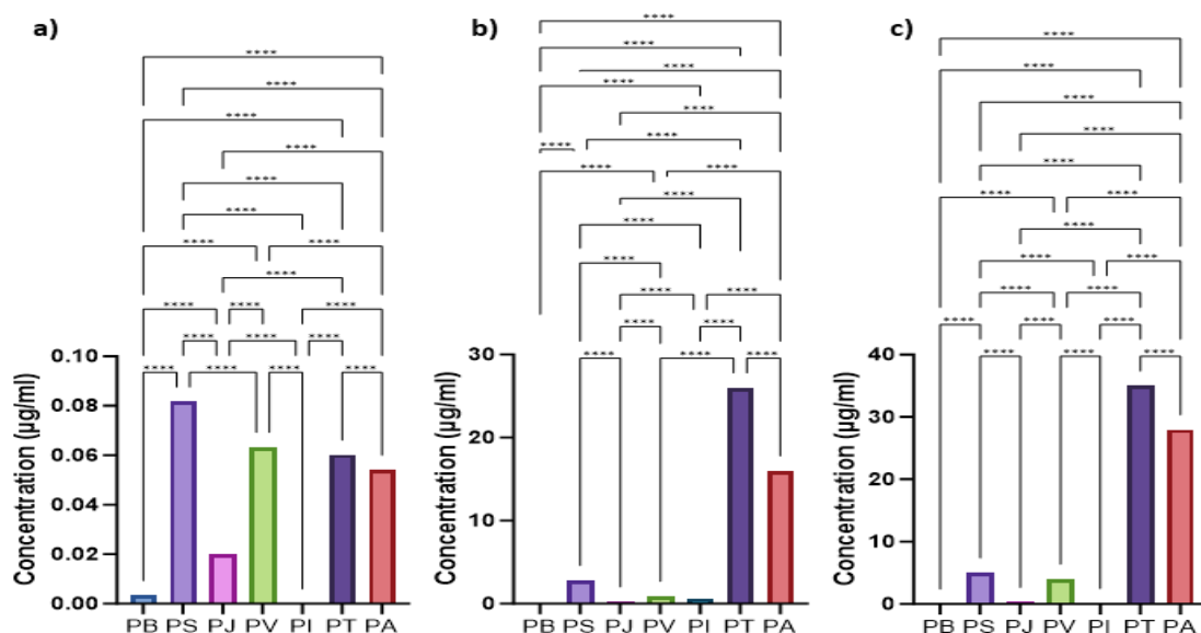
Figure (3): Comparable concentration values ( \mu\text{g/mL} ) of Al (a), Zn (b), and Cu (c) detected from seven natural oil products from different origins. All samples were analyzed by ICP-OES spectrometer following their digestion with the closed-microwave method. Data points represent concentration mean \pm SD ( n = 3 ). Significant differences of the same detected element between the different fish oil products are expressed as **** P < 0.0001 .
