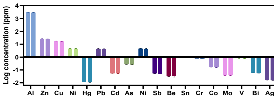
Figure (1): Summary of concentration values (ppm) of 18 elements analyzed by ICP-OES spectrometer of certified reference material GBW07605 tea sample. Samples were analyzed after using both the closed-microwave (first column) and the open-wet (second column) digestion methods. Data points represent log concentration mean \pm SD (n = 3). Considering the significant statistical significance of p \leq 0.05 ; no significant differences were detected between the two used digestion methods for the same detected element.
