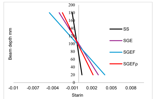
Figure (11): Concrete strain with height of the beam.
