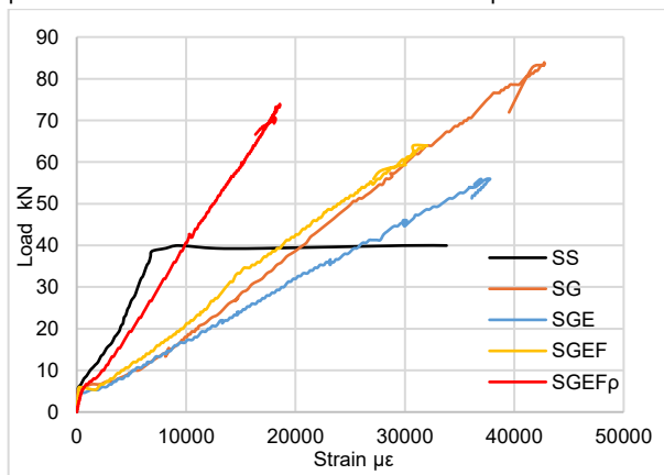
Figure (9): Load - strain of the rebars.
