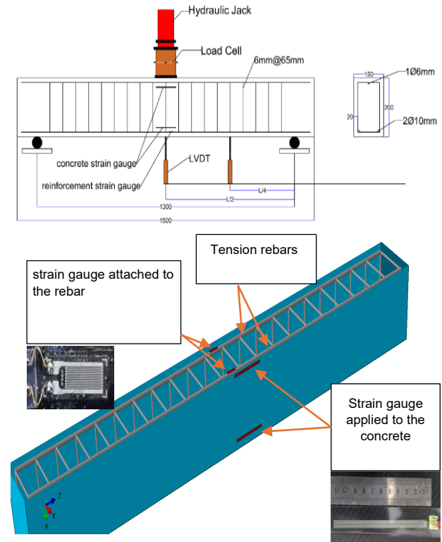
Figure (3): Details of reinforcement bars and equipment.
