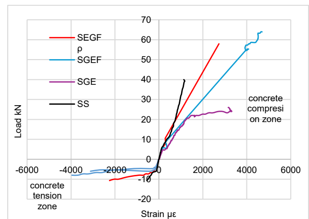
Figure (10): Load-strain of concrete beams.
