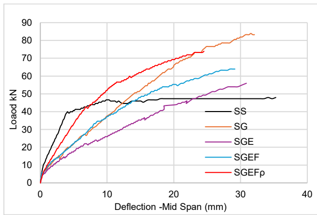
Figure (8): Load-deflection curves.
