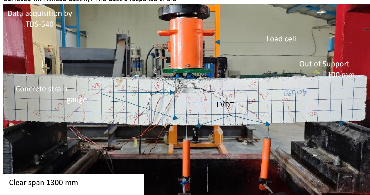
Figure (7): The test setup.
