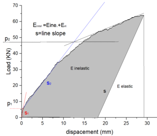
Figure (13): Example of the ductility index for beam SGE.
