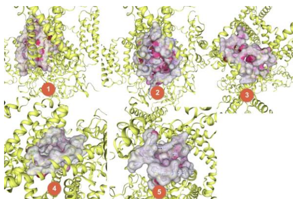
Figure (3): Cavities detected in protein SCN1A.
