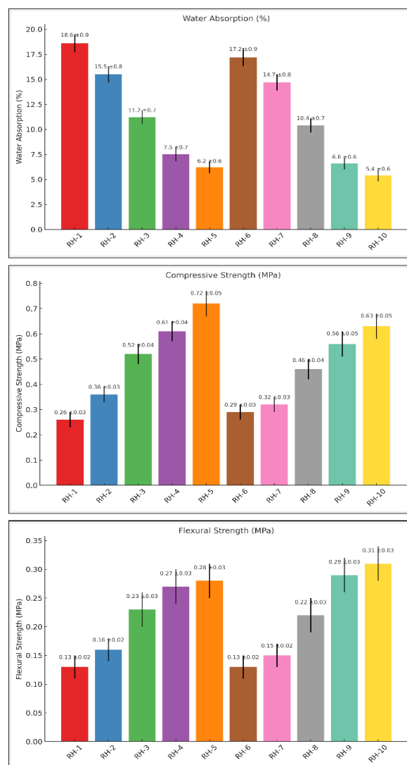
Figure (5): Water Absorption and Mechanical Results.
