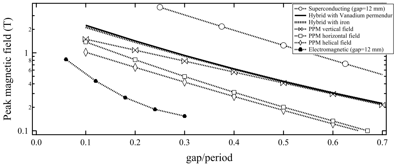
FIG. 3: Peak magnetic field as a function of the gap to period ratio ( g/\lambda_0 ) for different wiggler technologies.
