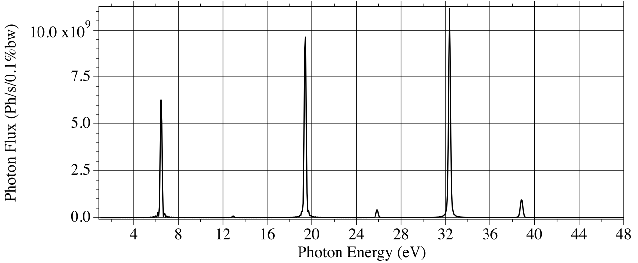
FIG. 6: Photon flux of the first proposed wiggler ( \lambda_0 = 98 mm) in the undulator regime calculated by SRW at 10 m from the source through an aperture of 0.1 \times 0.1 mm 2 . The wiggler is set at gap 16.7 mm. The magnetic field B=1.63 T. The electron beam parameters are: E = 2.739 GeV, I = 500 mA, \beta_x = 4.6 m, \beta_z = 2.2 m, \epsilon_x = 3.9 nm.rad, \epsilon_z = 39 pm.rad, \sigma_e = 0.1\% .
