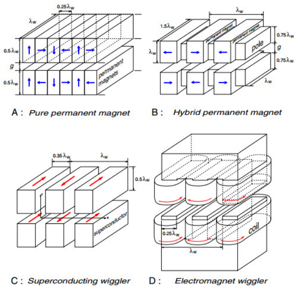
FIG. 1: Common magnetic designs and dimensions of insertion devices. Blue arrows indicate the magnetization direction, red arrows indicate the current direction [7].
