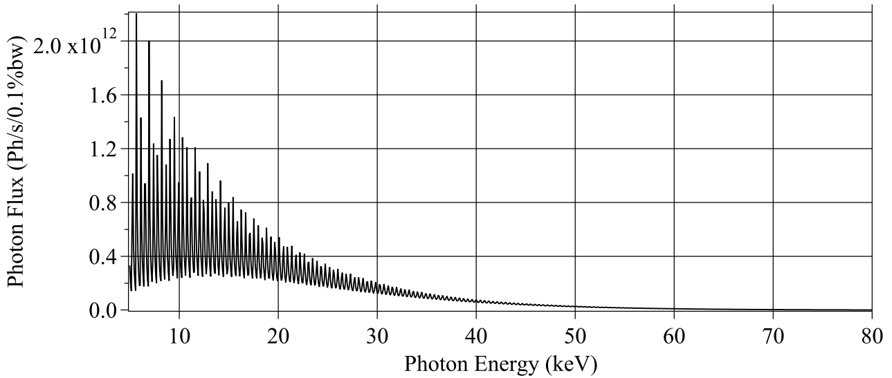
FIG. 7: Photon flux of the first proposed wiggler ( \lambda_0 = 98 mm) in the wiggler regime calculated by SRW at 10 m from the source through an aperture of 0.1 \times 0.1 mm 2 . The wiggler is set at gap 14.7 mm. The magnetic field B=1.78 T. The electron beam parameters are: E = 2.739 GeV, I = 500 mA, \beta_x = 4.6 m, \beta_z = 2.2 m, \epsilon_x = 3.9 nm.rad, \epsilon_z = 39 pm.rad, \sigma_e = 0.1\% .
