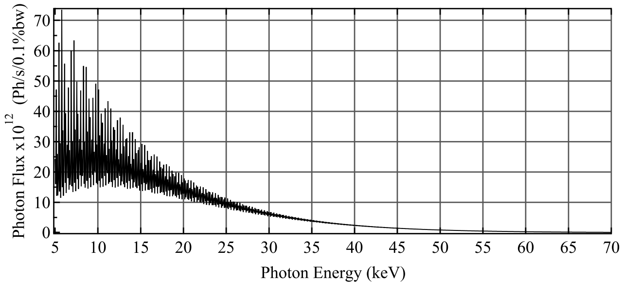
FIG. 5: Photon flux of the first proposed wiggler ( \lambda_0 = 164 mm) in the wiggler regime calculated by SRW at 10 m from the source through an aperture of 0.1 \times 0.1 mm 2 . The wiggler is set at gap 14.7 mm. The field B=1.65 T. The electron beam parameters are: E = 2.739 GeV, I = 500 mA, \beta_x = 4.6 m, \beta_z = 2.2 m, \epsilon_x = 3.9 nm.rad, \epsilon_z = 39 pm.rad, \sigma_e = 0.1\% .
