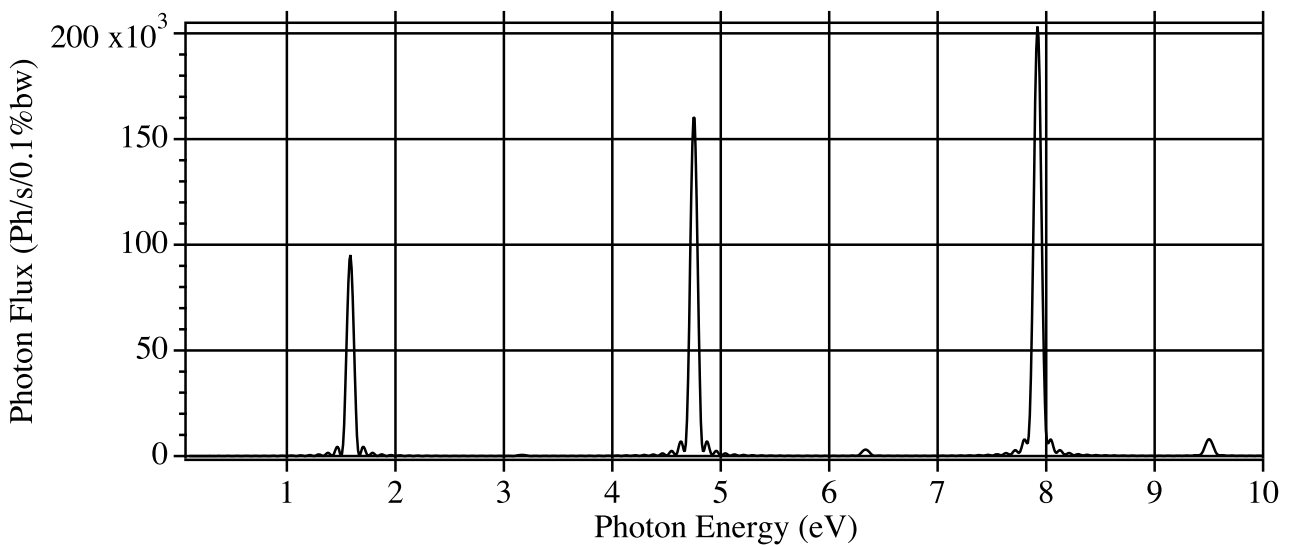
FIG. 4: Photon flux of the first proposed wiggler ( \lambda_0 = 164 mm) in the undulator regime calculated by SRW at 10 m from the source through an aperture of 0.1 \times 0.1 \text{ mm}^2 . The wiggler is set at gap 16.7 mm. The magnetic field B=1.52 T. The electron beam parameters are: E = 2.75 GeV, I = 500 mA, \beta_x = 4.6 m, \beta_z = 2.2 m, \epsilon_x = 3.9 nm.rad, \epsilon_z = 39 pm.rad, \sigma_e = 0.1\% .
