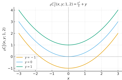
Figure 1: Graph of {}_EC_2^1(x, y; 1, 2) = \frac{x^2}{3} + y for y = -1, 0, 1 . Each curve represents a parabola shifted vertically by y .
