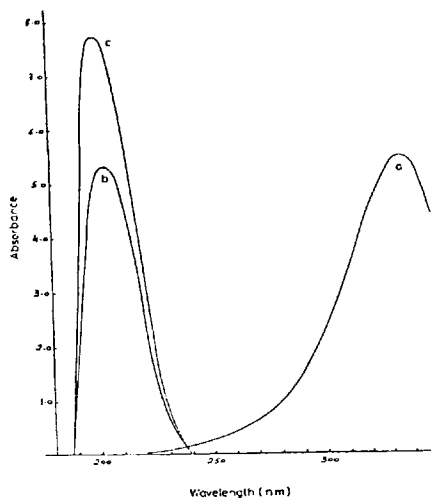
Fig. 1 Absorption spectra of PAPH and its complexes :
