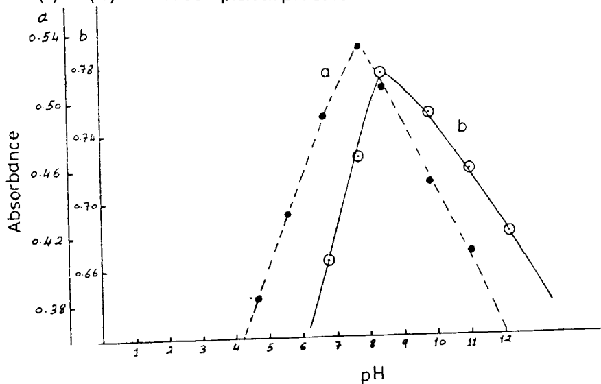
Fig.2 pH dependence of metal complexes :
